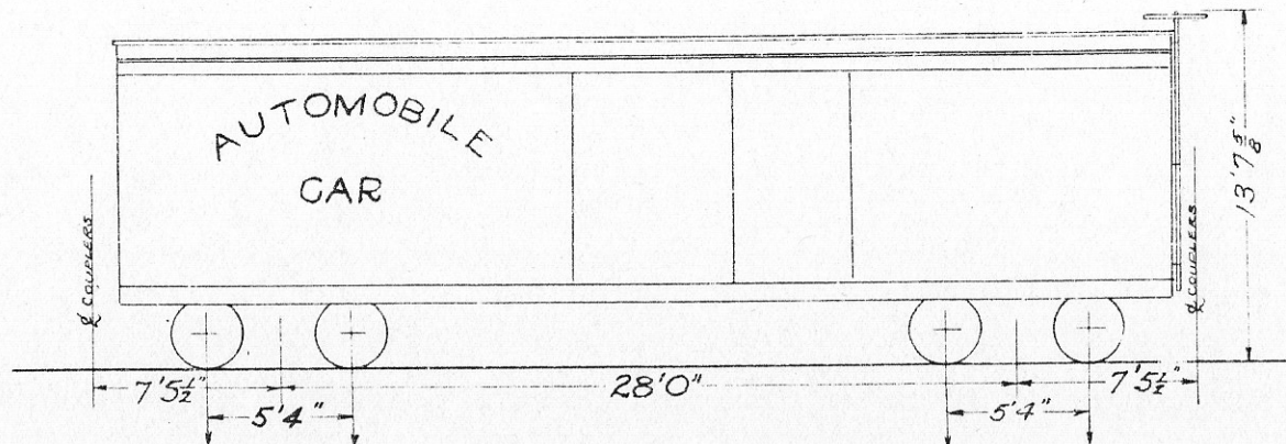
A.R.R. - 1100 SERIES AUTOMOBILE CAR
